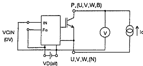
Fig.1 V_{CE(sat)} T_{set}
